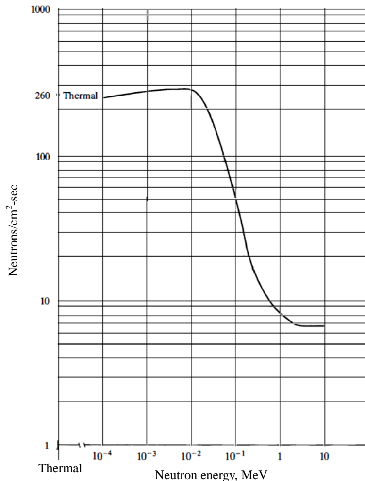
Neutron flux that gives dose-equivalent rate of 1 mrem/hr as a function of neutron energy. (Based on Appendix 6, ICRP Publication 21.)
